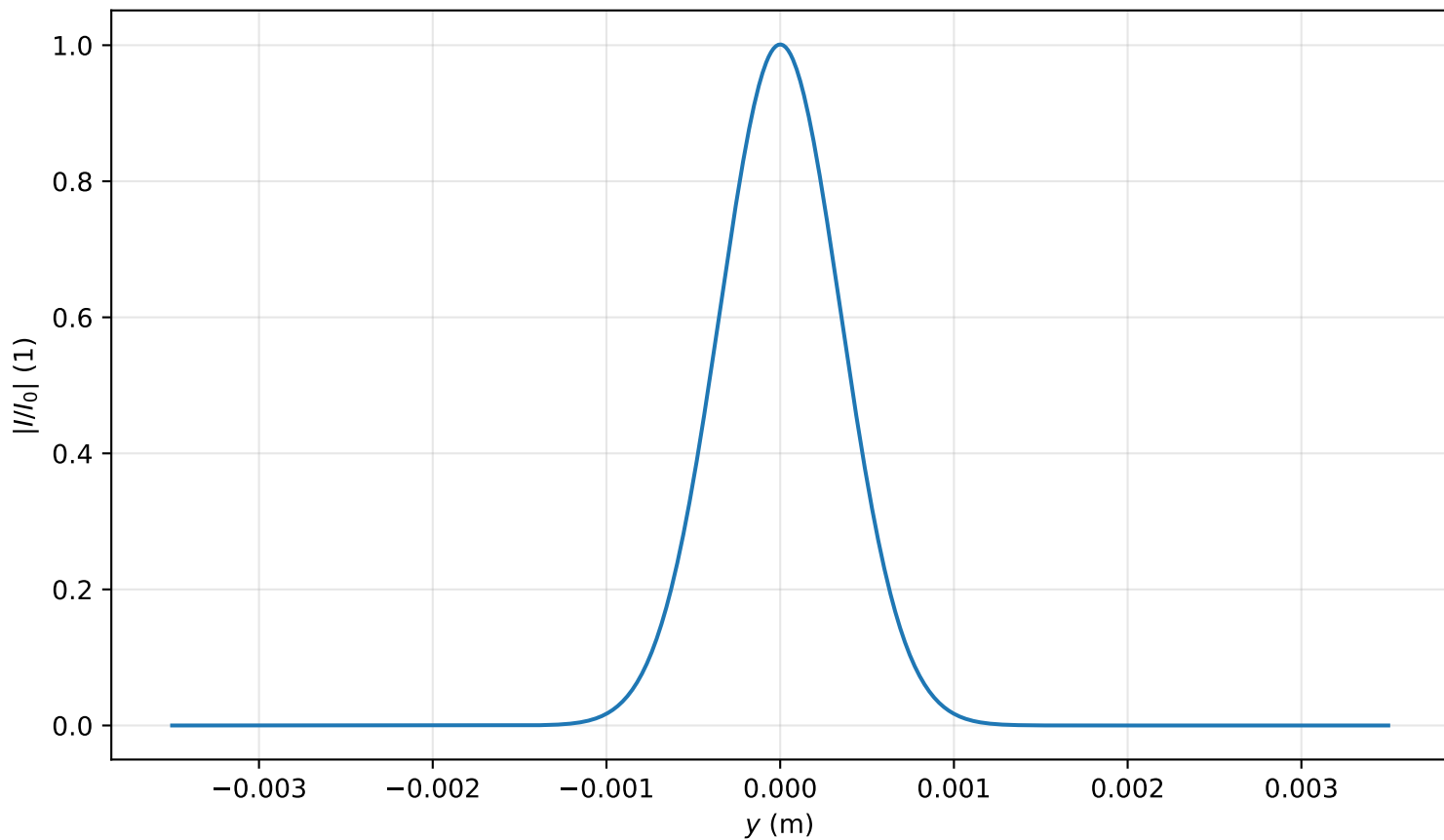
Intensity profile I(x=0, y, z=0.159)/I_0 , P_{in}=0.3P_{cr} , artificial time
